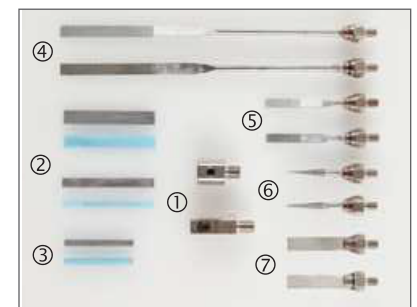
Standard and attachment tools.
