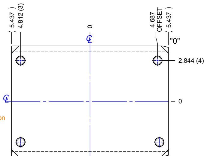
Cavity Plan View
