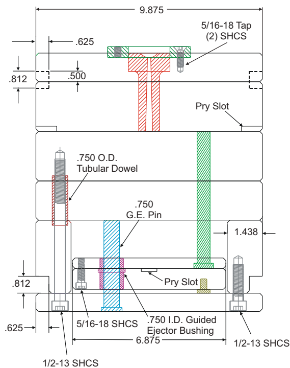
End View
