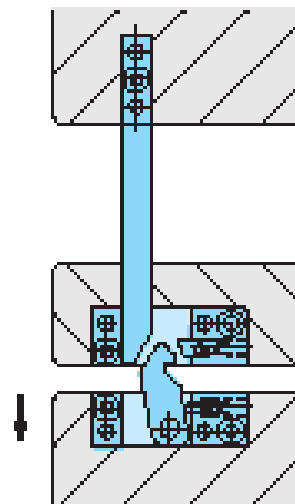
(Fig. 4) Parting Line is released
