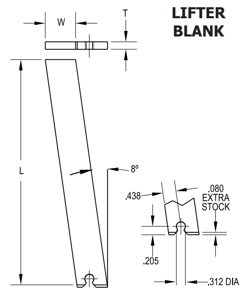
E-Z Lifter™ Standard Lifter Blank Table: Enter custom dimensions below
