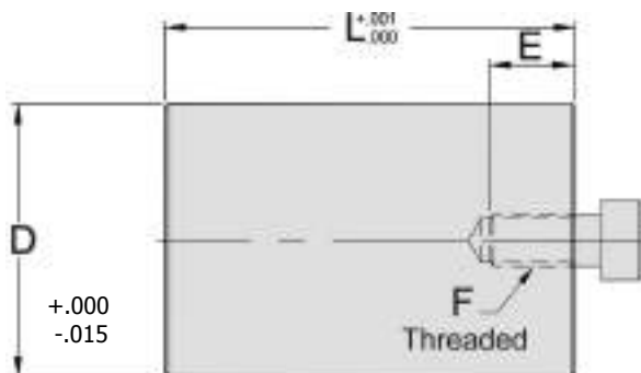
Threaded (Tapped Hole) Support Pillar Enter custom dimensions below
