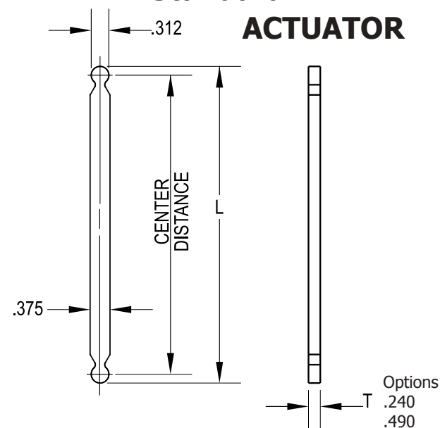
E-Z Lifter™ Standard Series Table: Enter custom dimensions below
