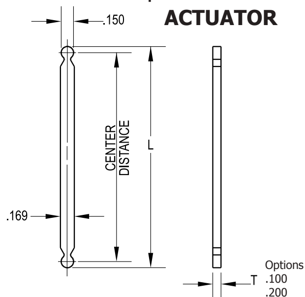
E-Z Lifter™ Mini Series Table: Enter custom dimensions below
