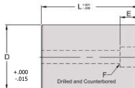
Drilled & Counterbored Support Pillar Enter custom dimensions below
